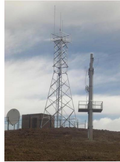
Skytel 20 m Tower, 4x4 shelter, Uvs Province
