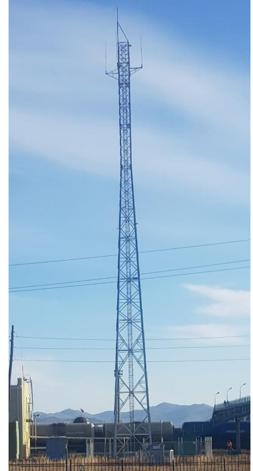
70 m Tower, Ulaanbaatar railway, Selenge Province
